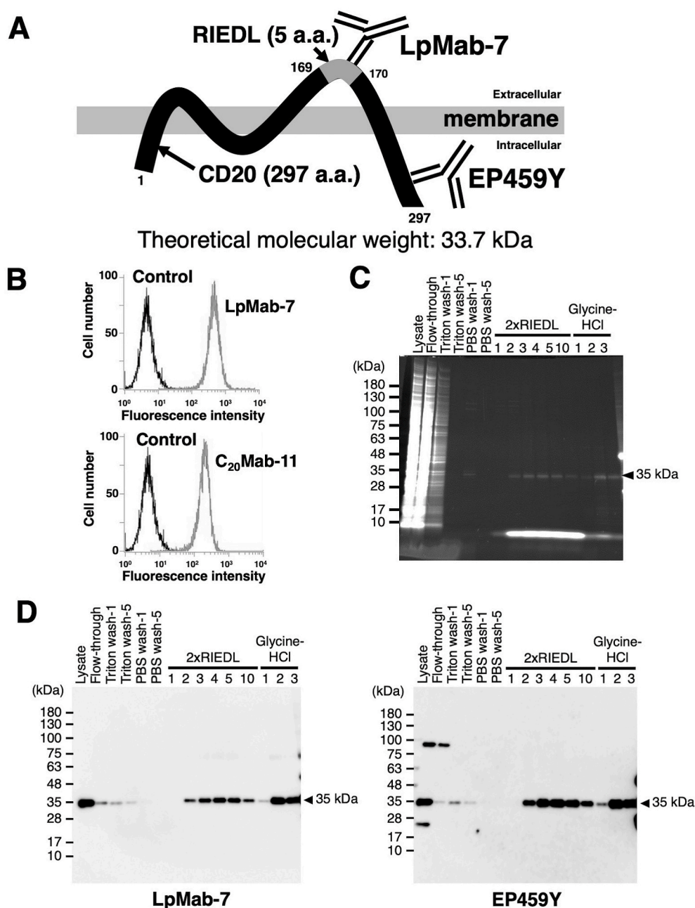
Fig. 2. Purification of CD20-169RIEDL 170 using the RIEDL tag system. (A) Schematic illustration of CD20-169RIEDL 170 . The epitopes of LpMab-7 and anti-CD20 mAb (clone EP459Y) are indicated. (B) Flow cytometry using an anti-RIEDL tag mAb. CHO/CD20-169RIEDL 170 was detected by anti-RIEDL tag mAb (LpMab-7, upper panel) and anti-CD20 mAb (C 20 Mab-11, lower panel). (C) Cell lysates (Lysate) were loaded onto an LpMab-7-Sepharose column, and unbound proteins passed through (flow-through). After five washes with PBS containing Triton X-100 (Triton wash-1 and Triton wash-5) and five washes with PBS (PBS wash-1 and PBS wash-5), bound proteins were eluted with 2 × RIEDL peptide (2 × RIEDL 1–5, and -10) followed by acidic buffer (glycine-HCl 1–3). Elution fractions were applied to SDS-PAGE, and the gel was stained with Oriole Fluorescent Gel Stain. (D) Elution fractions from the column chromatography were applied to SDS-PAGE, and the proteins were transferred to PVDF membranes. The membranes were immunostained with 1 µg/ml of an anti-RIEDL tag mAb (LpMab-7; left panel) or an anti-CD20 mAb (clone EP459Y; right panel) and incubated with peroxidase-conjugated secondary antibody specific for mouse immunoglobulins.
